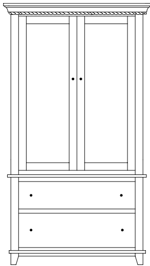
BK-2862 Armoire 42"w 76¼"h 22¼"d w/2 drawers, w/2 doors, 2 adj. shelves & closet rod
