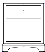
MR-4104 1 Drawer Overall Width: 25" Overall Depth: 19" Height: 28¾"
