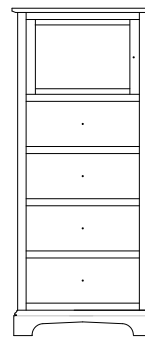
MR-4127 4 Drawer, 1 Door Lingerie Chest Overall Width: 25" Overall Depth: 19" Height: 58"
